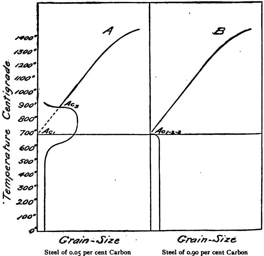
Fig. 77. Conjectured Relation between Temperature and Size of Grain of Steel. First Approximation.
